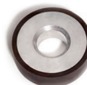
MMS 130400 Diameter 130mm Chamfer diameter 115mm Width 40mm Bore 50mm Universal Roller with chamfered hub for CEREX machines
